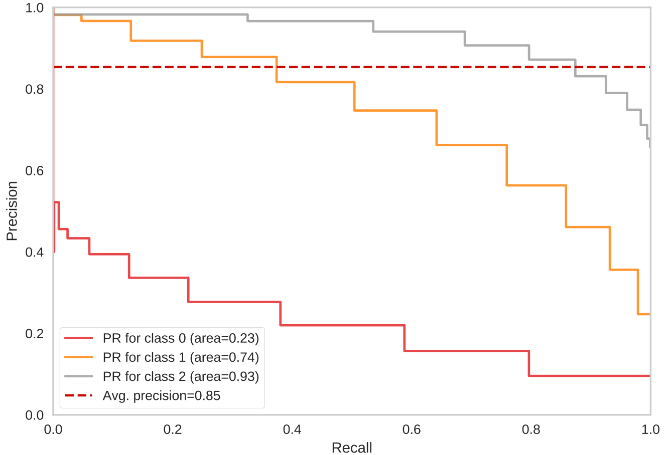
Precision-Recall Curve for RandomForestClassifier
