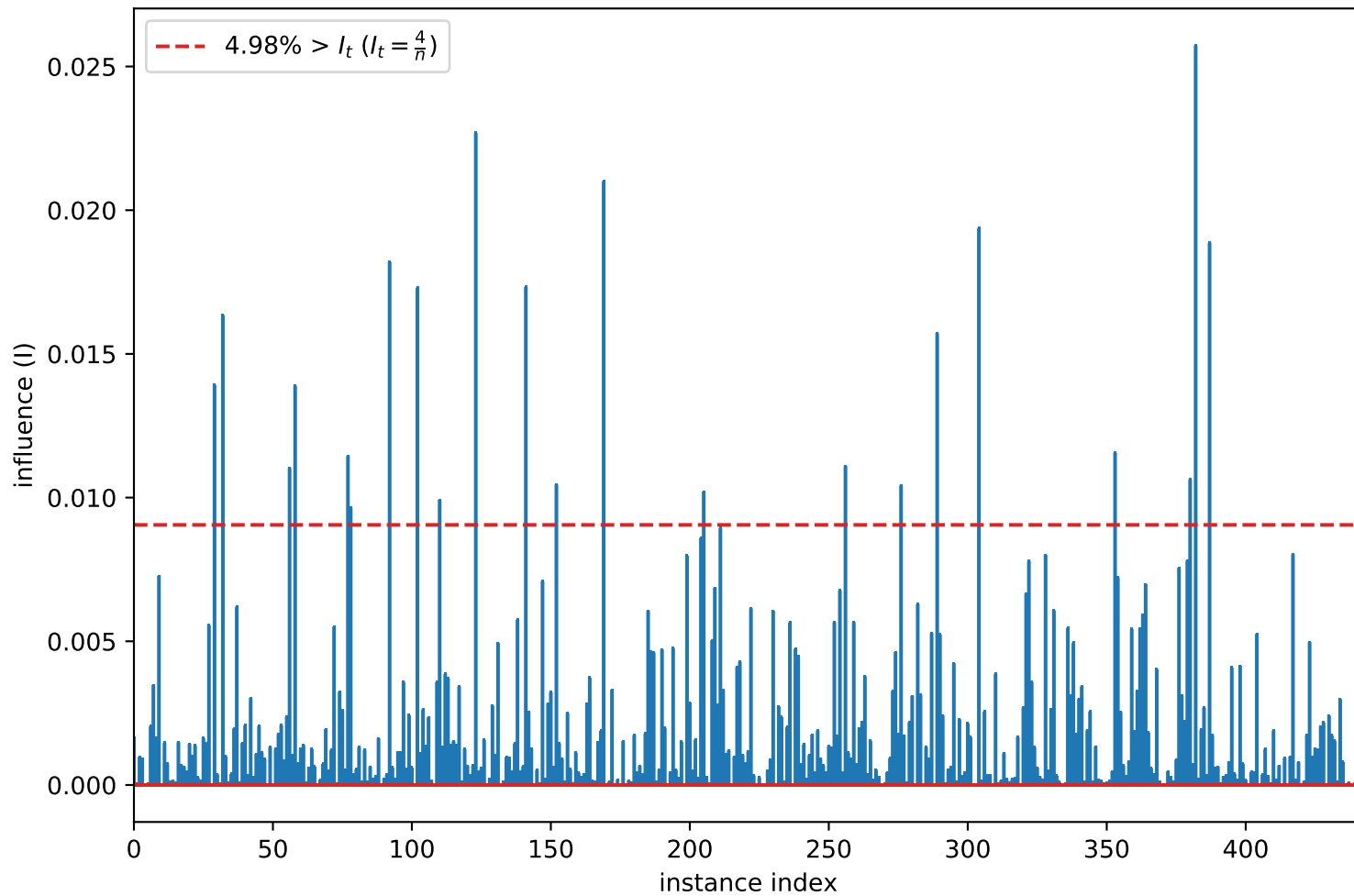
Cook's Distance Outlier Detection
