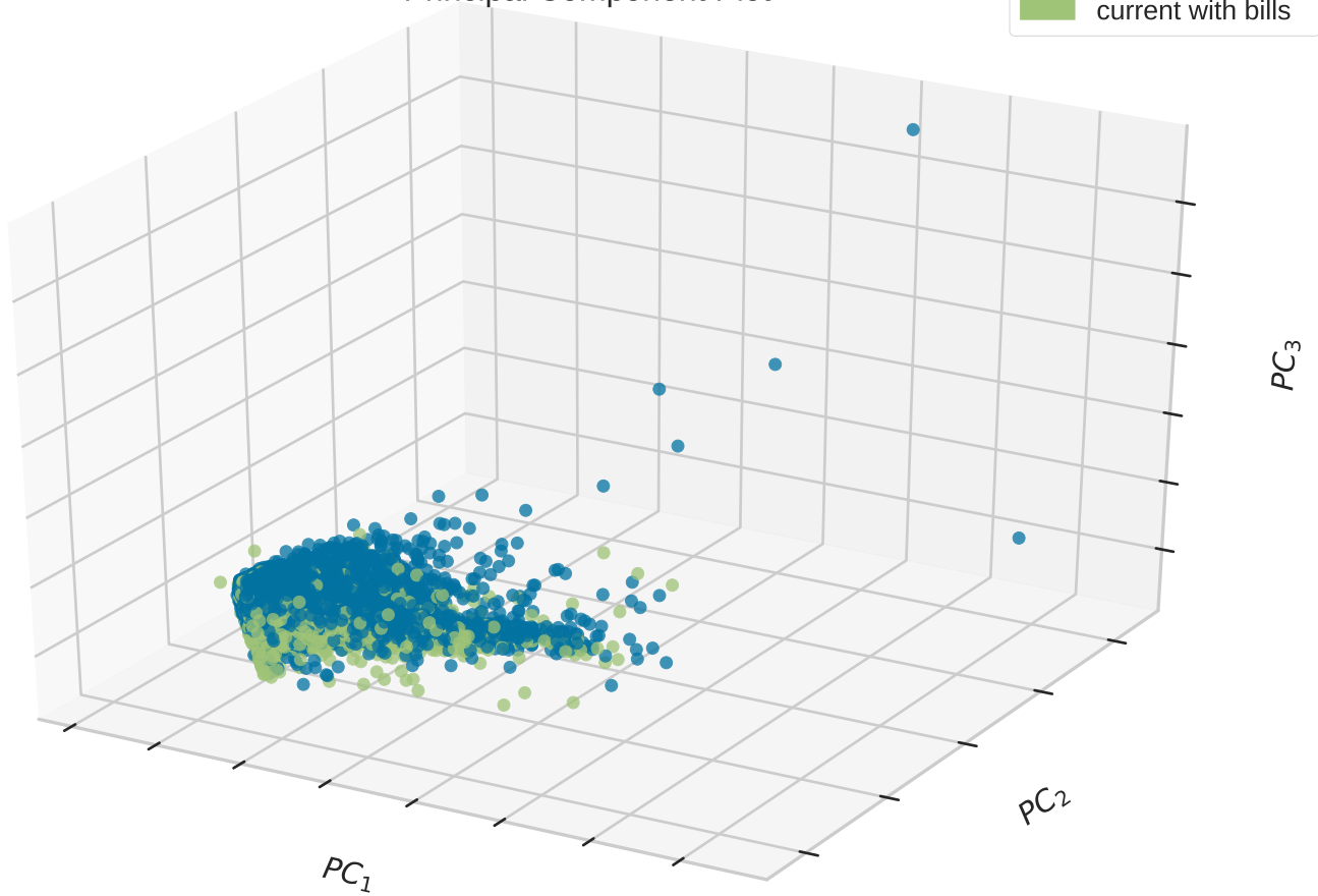
Principal Component Plot
