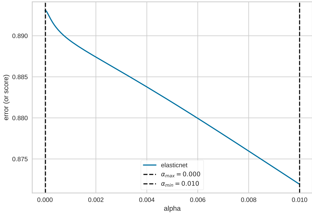
ElasticNet Alpha Error
