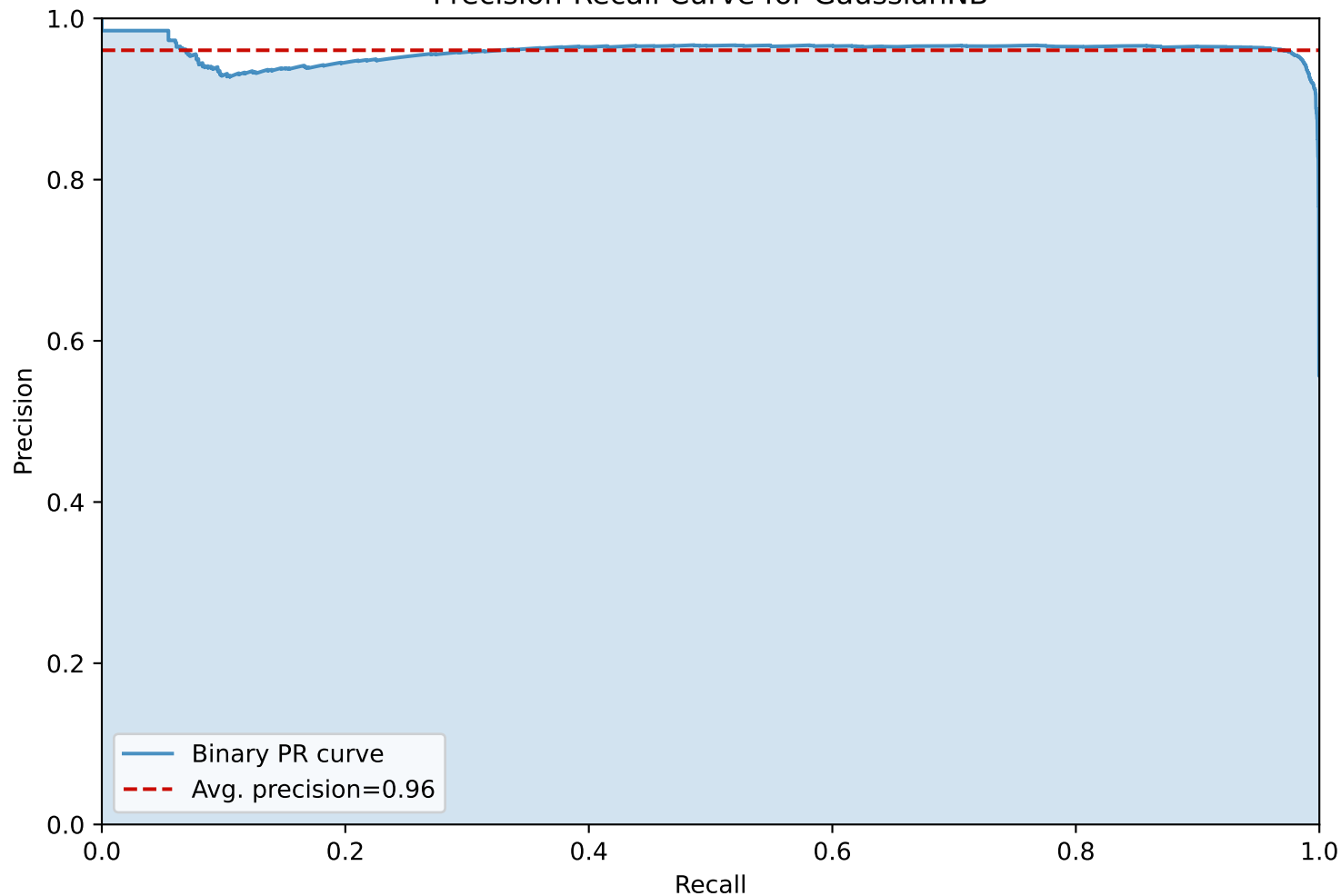
Precision-Recall Curve for GaussianNB
