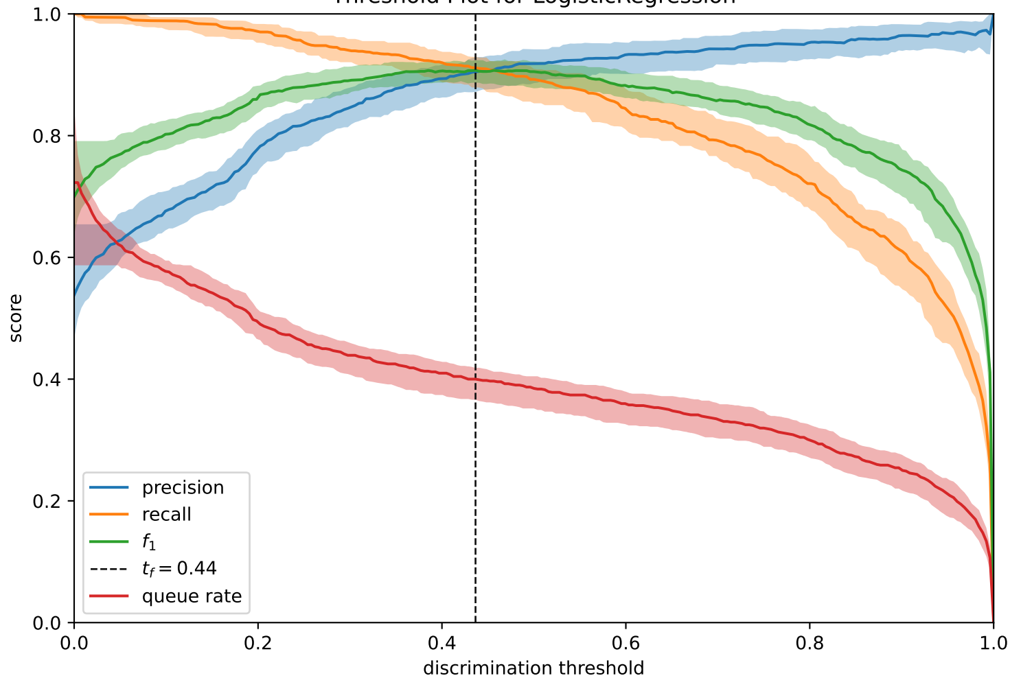
Threshold Plot for LogisticRegression
