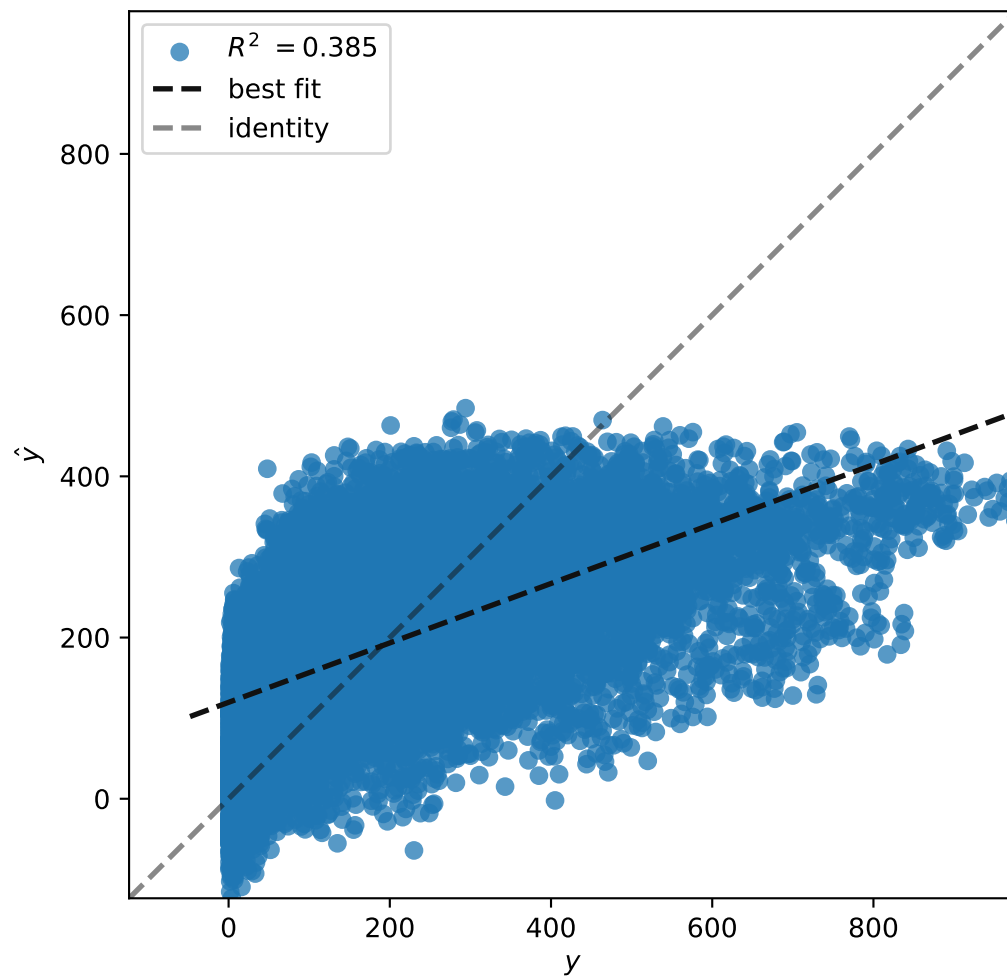
Prediction Error for Lasso
