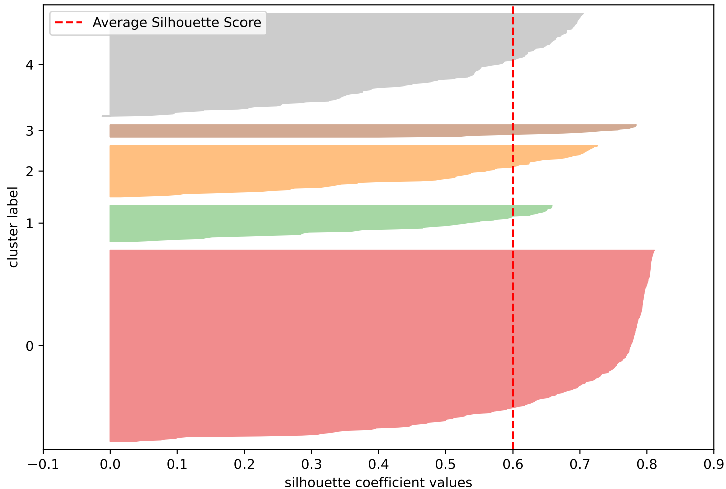
Silhouette Plot of KMeans Clustering for 494 Samples in 5 Centers
