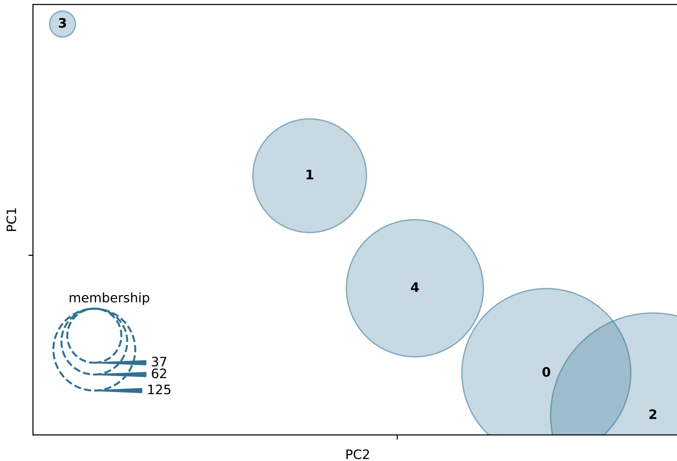
MiniBatchKMeans Intercluster Distance Map (via MDS)
