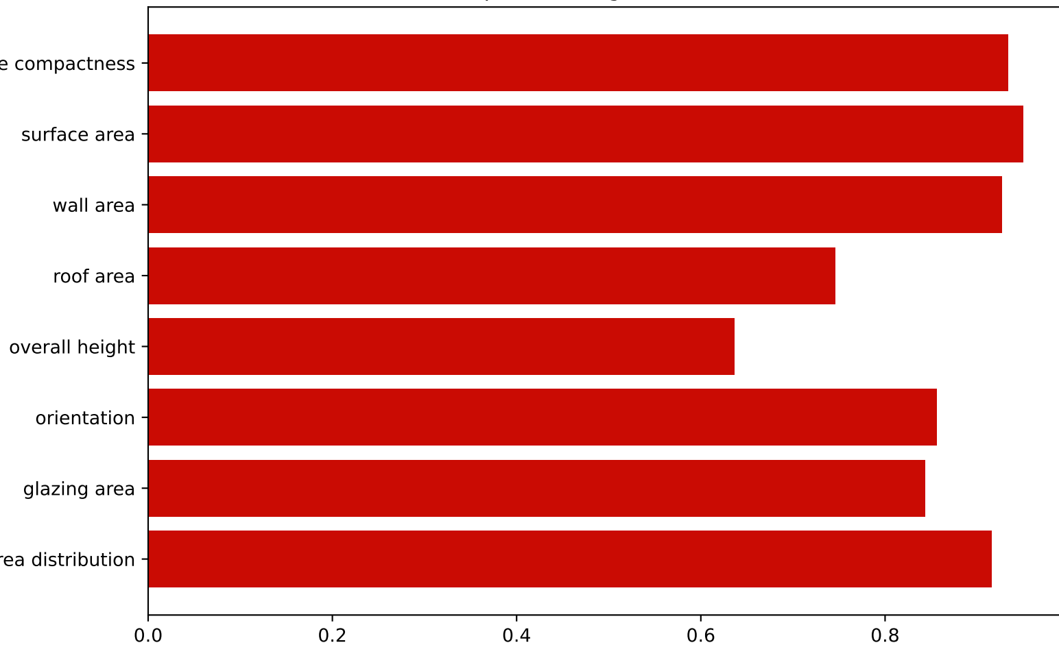
Shapiro Ranking of 8 Features
