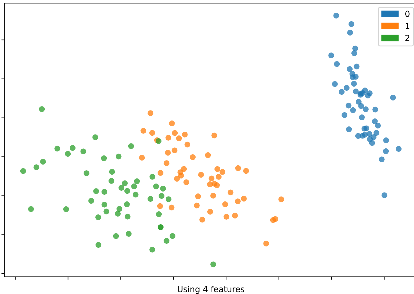
MDS Manifold (fit in 0.29 seconds)
