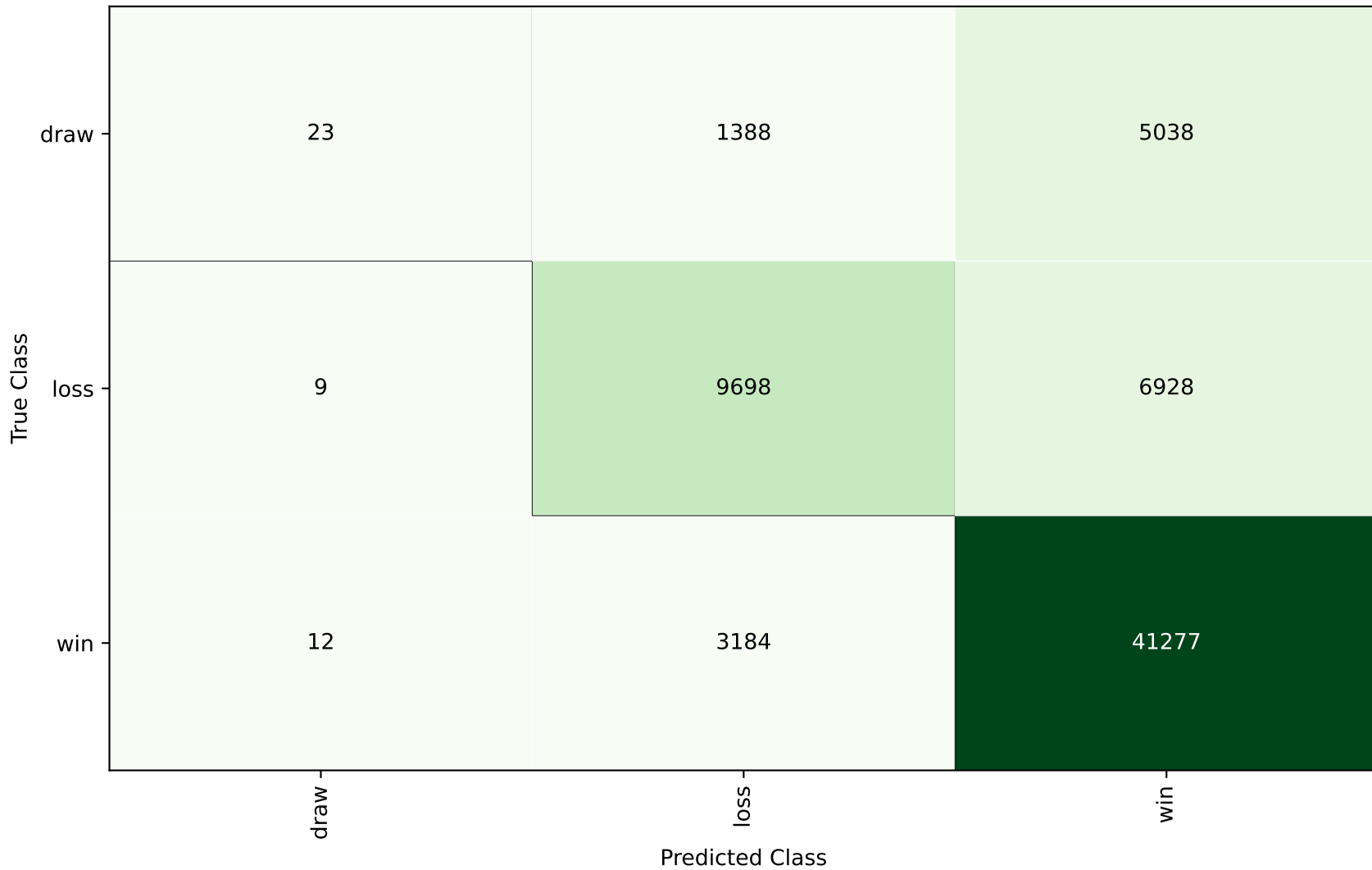
RidgeClassifier Confusion Matrix
