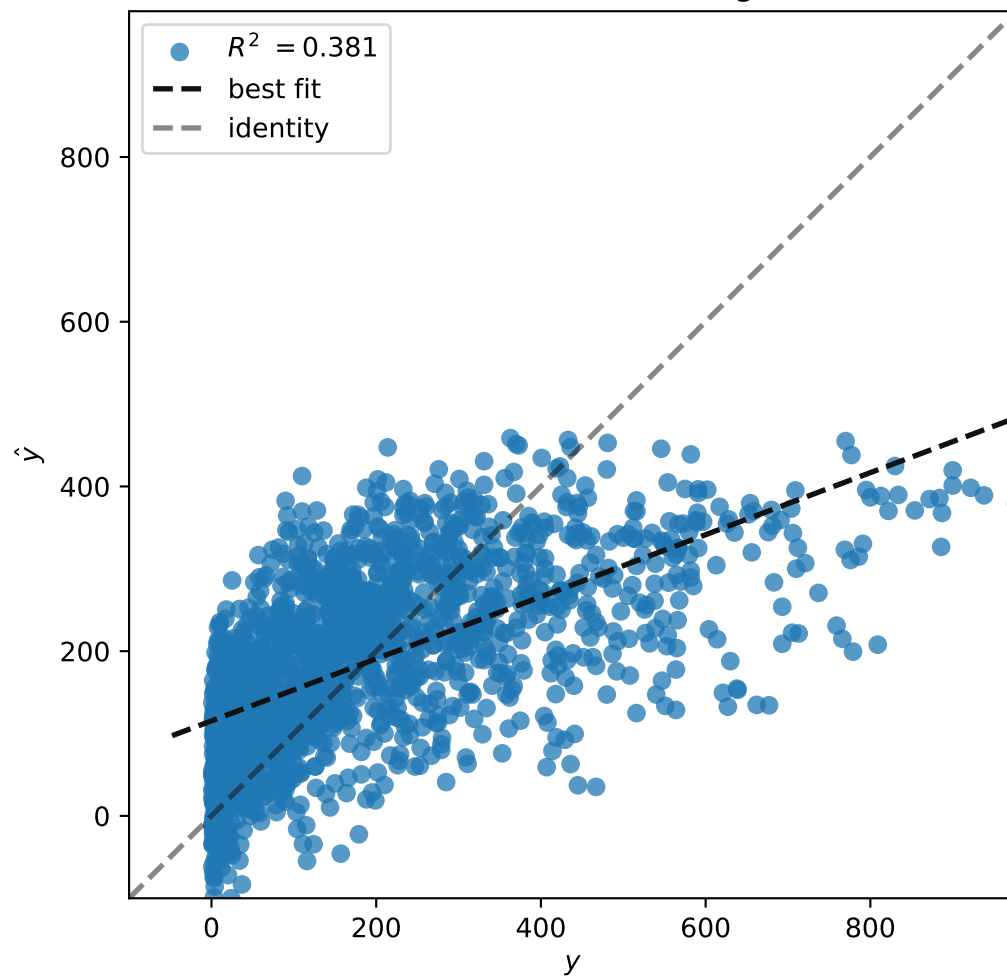
Prediction Error for Ridge
